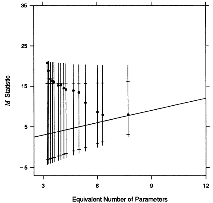
Figure 12. Abrasion-Loss Data. Figure 11 suggests that an additive nonparametric smoothing with no interaction will fit the data. This figure is an M plot for additive fits with hardness estimated by linear least squares and abrasion loss estimated by loess, with f ranging from .3 to 1 in steps of .05. On the basis of this plot, f was chosen to be .75.
