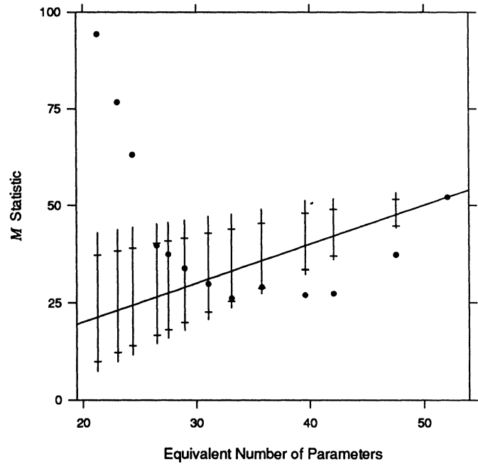
Figure 14. \text{NO}_x Data. The data are from an experiment studying the dependence of \text{NO}_x exhaust emissions on equivalence ratio, compression ratio, and type of fuel. The figure is an M plot for locally quadratic fitting, with f ranging from .4 to 1 in steps of .05. The type of fuel and the level of compression ratio, which took on one of five values, were both entered as categorical variables. On the basis of the plot, f was chosen to be .85.
